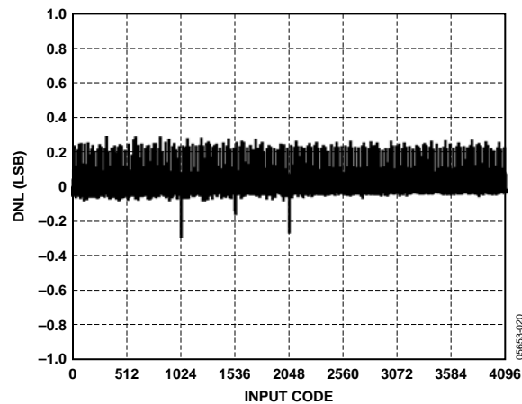
Figure 10. DNL vs. Code @ T_A = 25^\circ\text{C} , \text{INV} = L
