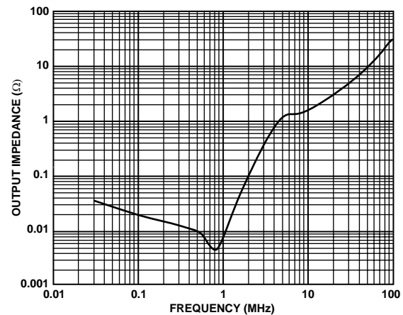
Figure 9. Output Impedance vs. Frequency; \text{PWN} = (1,1)
