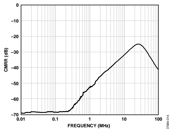
Figure 12. CMRR vs. Frequency; V_{IN} = 200\text{ mV p-p} , Gain = 10, I_{ADJ} = NC
