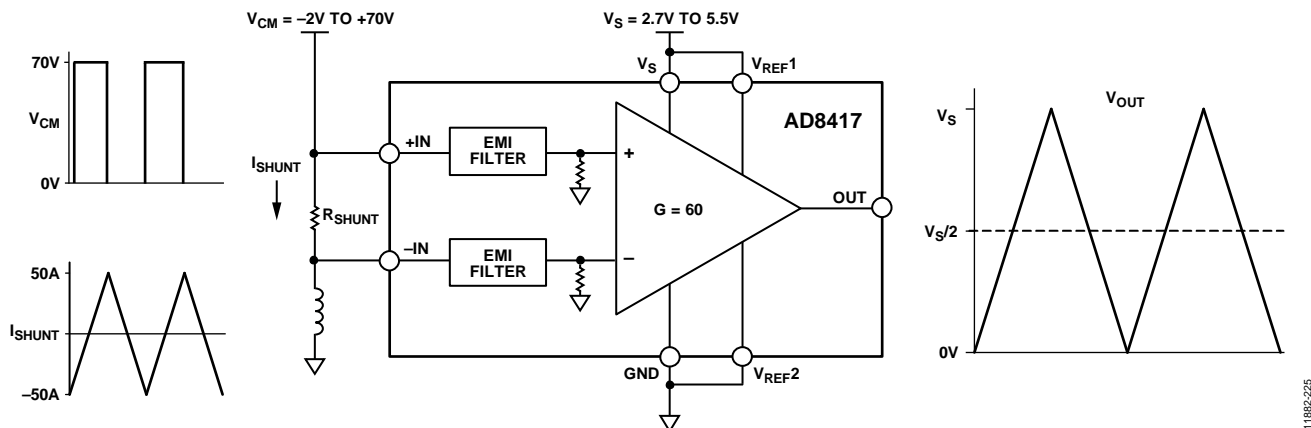
Figure 26. Typical Application
