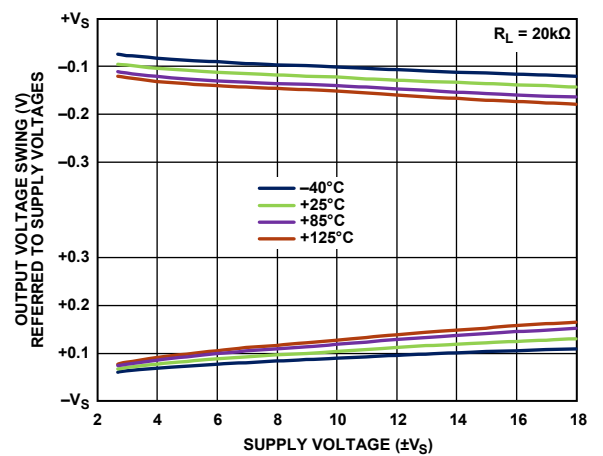
Figure 38. Output Voltage Swing vs. Supply Voltage, R_L = 20 kΩ
