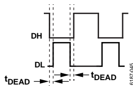
Figure 46. Dead Time ( t_{\text{DEAD}} ) Between DH and DL Transitions
