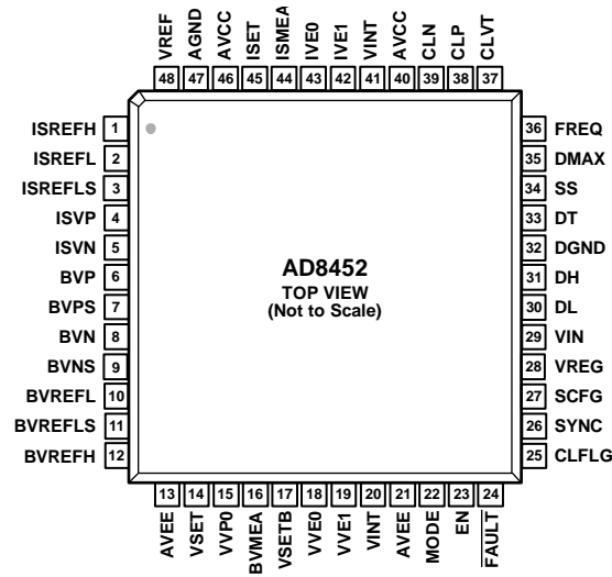
Figure 2. Pin Configuration
