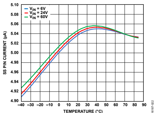
Figure 22. SS Pin Current vs. Temperature
