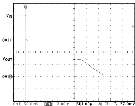
Figure 43. Positive Overload Recovery (Gain = 70)
