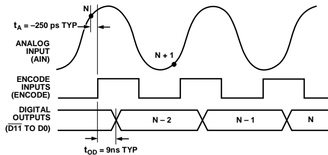
Figure 19. Timing Diagram
