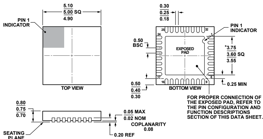
Figure 54. 32-Lead Lead Frame Chip Scale Package [LFCSP_WQ] 5 mm × 5 mm Body, Very Very Thin Quad (CP-32-12)
