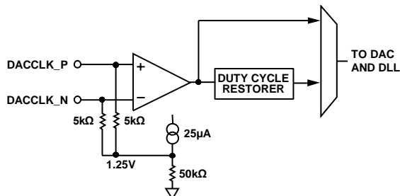
Figure 147. Clock Input
