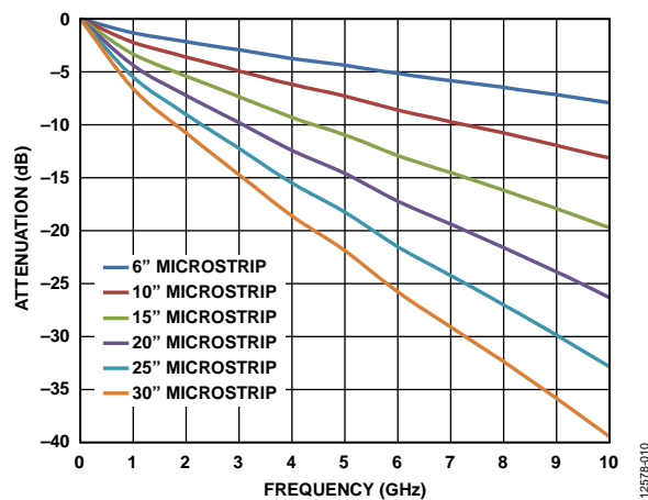
Figure 49. Insertion Loss of 50 Ω Microstrips on FR4
