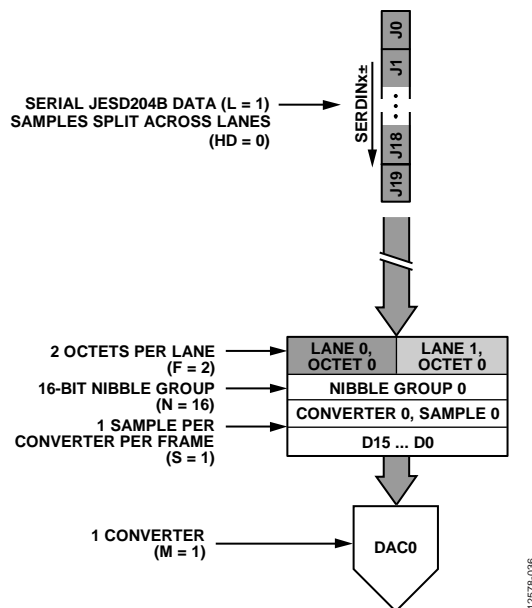
Figure 64. JESD204B Mode 10 Data Deframing
