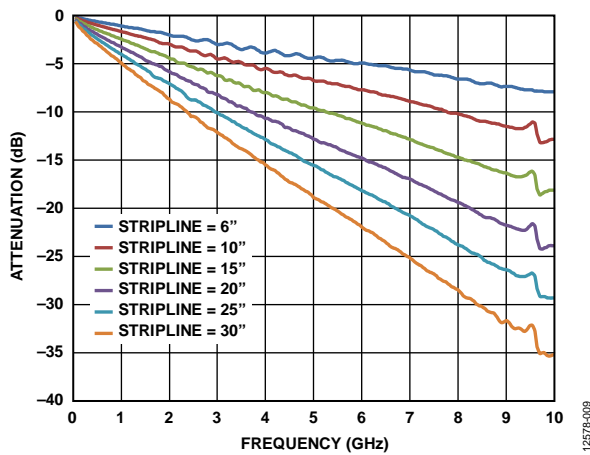
Figure 48. Insertion Loss of 50 Ω Striplines on FR4
