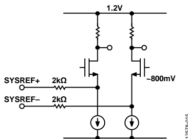
Figure 53. SYSREF± Input Circuit
