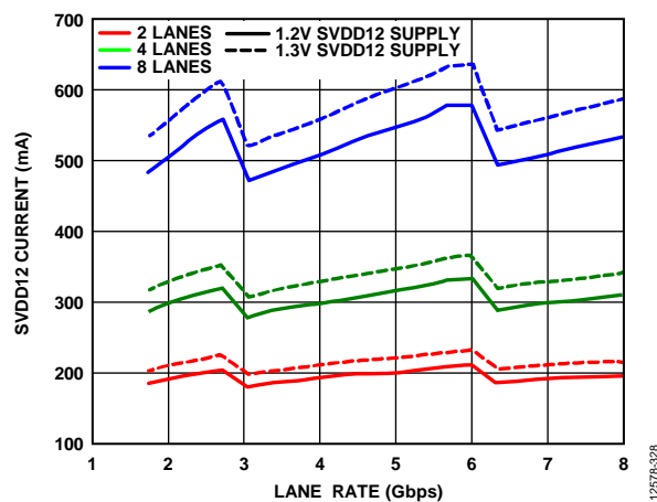
Figure 36. SVDD12 Current vs. Lane Rate over Number of SERDES Lanes and Supply Voltage Setting
