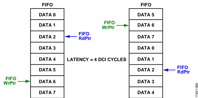
Figure 64. Example of Equal FIFO Latencies
