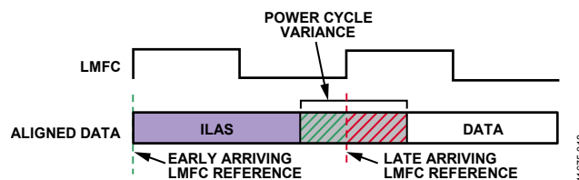
Figure 46. Link Delay > LMFC Period Example
