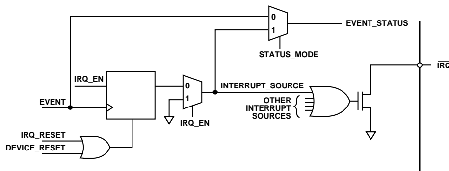
Figure 75. Simplified Schematic of IRQ Circuitry
