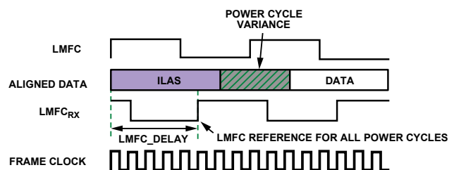
Figure 47. LMFC_DELAY to Compensate for Link Delay > LMFC
