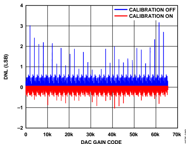
Figure 83. Pre-Calibration and Post-Calibration, DNL
