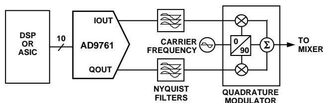
Figure 31. Typical Analog QAM Modulator Architecture
