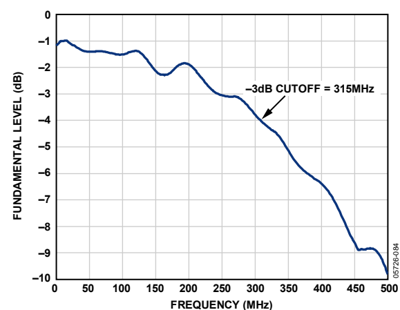
Figure 42. Full-Power Bandwidth vs. Frequency, f_{\text{SAMPLE}} = 65 \text{ MSPS}
