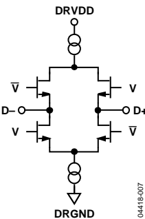
Figure 7. Equivalent Digital Output Circuit
