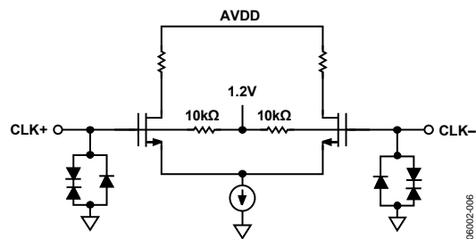
Figure 6. Clock Inputs
