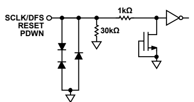
Figure 8. Equivalent SCLK/DFS, RESET, PDWN Input Circuit
