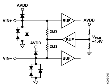
Figure 7. Analog Inputs ( V_{CML} \approx 1.4\text{ V} )
