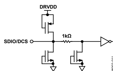
Figure 11. Equivalent SDIO/DCS Input Circuit
