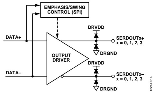
Figure 55. Digital Outputs
