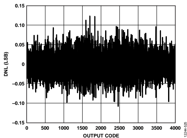
Figure 48. DNL, f_{IN} = 10 MHz
