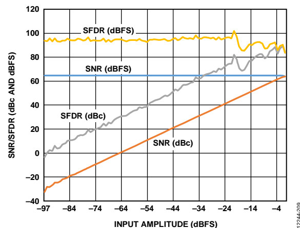
Figure 22. SNR/SFDR vs. Analog Input Level, f_{IN} = 10.3\text{ MHz} ; Buffer Current = 2.0\times
