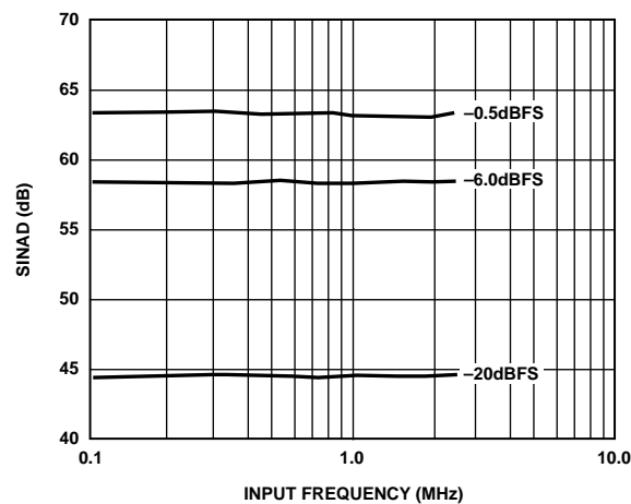
Figure 44. SINAD vs. Input Frequency ( f_{\text{CLOCK}} = 10 \text{ MSPS} )
