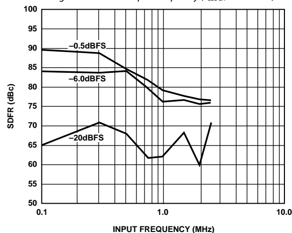
Figure 46. SFDR vs. Input Frequency ( f_{\text{CLOCK}} = 10 \text{ MSPS} )
