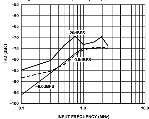
Figure 45. THD vs. Input Frequency ( f_{\text{CLOCK}} = 10 \text{ MSPS} )
