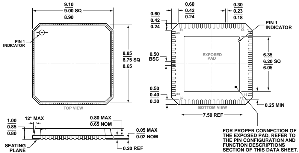
Figure 60. 64-Lead Lead Frame Chip Scale Package [LFCSP_VQ] 9 mm × 9 mm Body, Very Thin Quad (CP-64-4) Dimensions shown in millimeters
