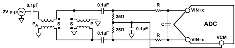
Figure 42. Differential Double Balun Input Configuration
