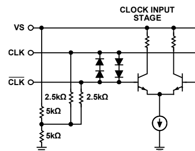
Figure 52. CLK Equivalent Input Circuit
