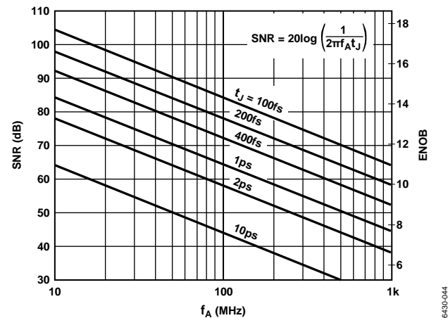
Figure 52. SNR and ENOB vs. Analog Input Frequency
