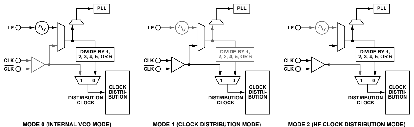
Figure 51. Simplified Diagram of the Three Clock Distribution Operation Modes
