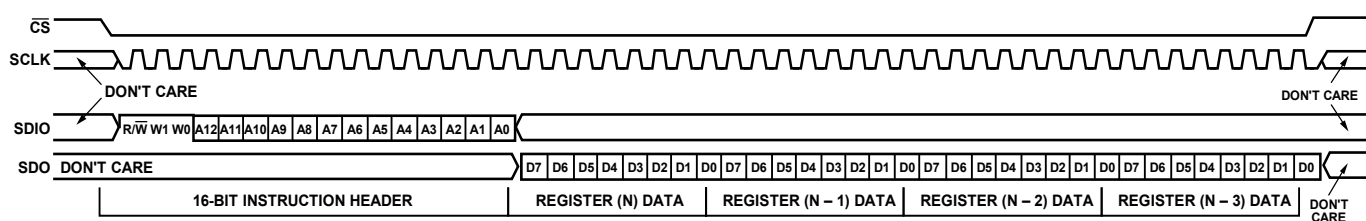
Figure 39. Serial Control Port Read—MSB First, 16-Bit Instruction, Four Bytes of Data
