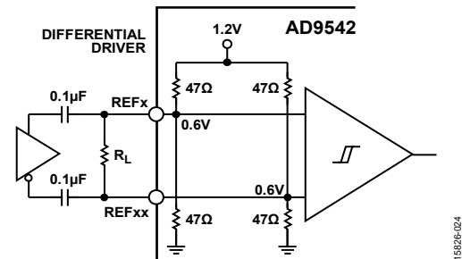
Figure 29. Differential AC-Coupled Mode ( R_L = 100 \Omega Is Recommended, Except For HCSL)
