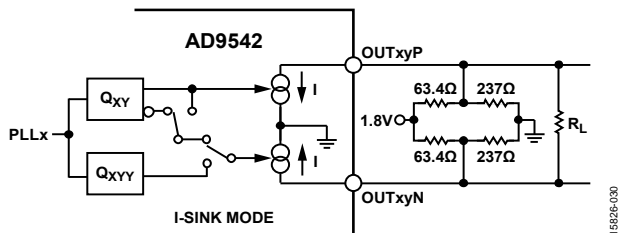
Figure 35. LVDS-Compatible Output, 1.2 V Common-Mode, Thevenin Bias Network ( I = 7.5 mA; 15 mA With Extra 100 Ω Termination, R_L )
