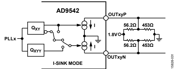
Figure 36. 2.5 V LVPECL or Double Amplitude LVDS-Compatible Boost Output, 1.5 V p-p , 1.24 V Common-Mode ( I = 15 mA)
