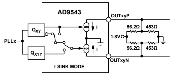
Figure 36. 2.5 V LVPECL or Double Amplitude LVDS-Compatible Boost Output, 1.5 V p-p , 1.24 V Common-Mode ( I = 15 mA)
