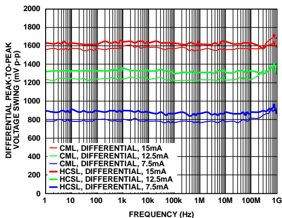
Figure 20. Differential Output Amplitude Waveforms; HCSL Drivers Terminated 50\ \Omega to GND per Figure 32; CML Drivers Terminated 50\ \Omega to 1.8 V per Figure 33
