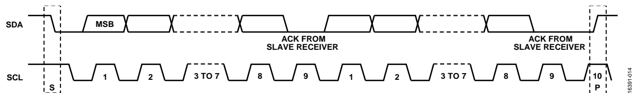
Figure 61. Acknowledge Bit
