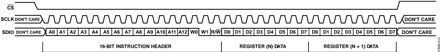
Figure 28. Serial Control Port Write—LSB First, 16-Bit Instruction, Two Bytes Data
