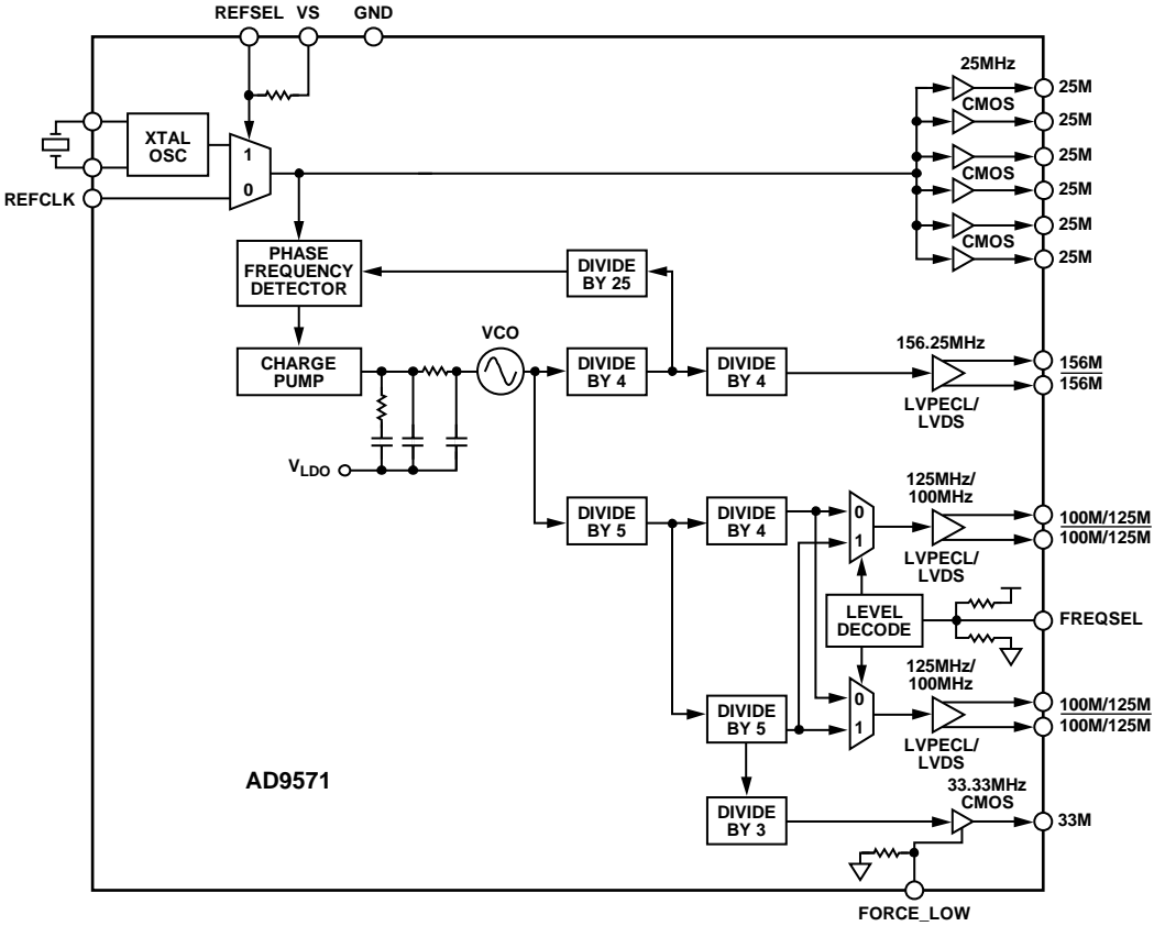
Figure 11. Detailed Block Diagram
