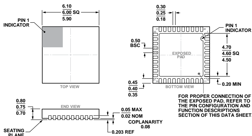
Figure 51. 40-Lead Lead Frame Chip Scale Package [LFCSP_WQ] 6 mm × 6 mm Body, Very Very Thin Quad (CP-40-7)
