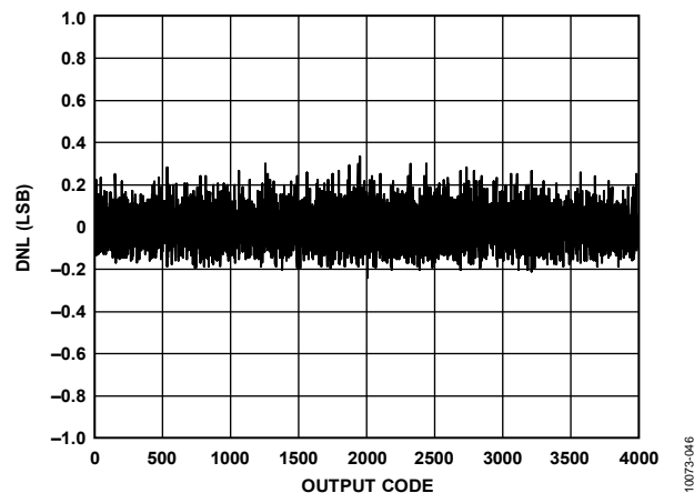
Figure 41. DNL, f_{IN} = 9.7 MHz, f_{SAMPLE} = 125 MSPS
