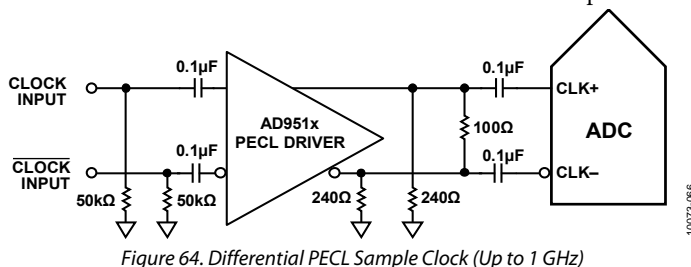
Figure 64. Differential PECL Sample Clock (Up to 1 GHz)
