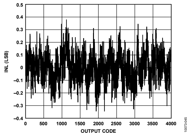
Figure 40. INL, f_{IN} = 9.7 MHz, f_{SAMPLE} = 125 MSPS
