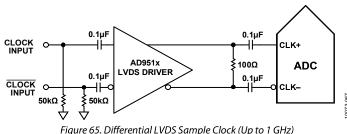
Figure 65. Differential LVDS Sample Clock (Up to 1 GHz)
