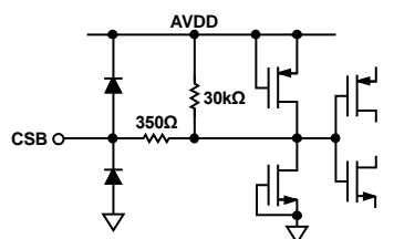
Figure 41. Equivalent CSB Input Circuit
