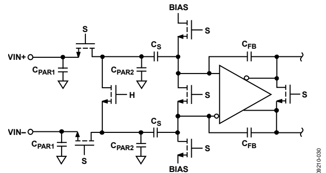
Figure 48. Switched-Capacitor Input
