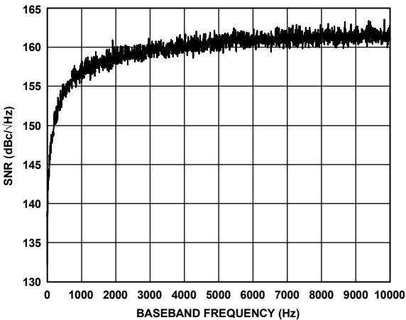
Figure 32. Output Referred SNR vs. Baseband Frequency
