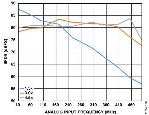
Figure 121. Buffer Current Sweeps, AD9680-1000 (SFDR vs. I_{BUFF} ); f_{IN} < 500\text{ MHz} ; Front-End Network Shown in Figure 115
