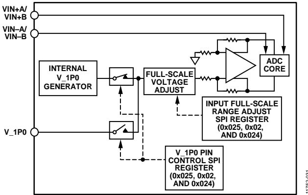
Figure 131. Internal Reference Configuration and Controls
