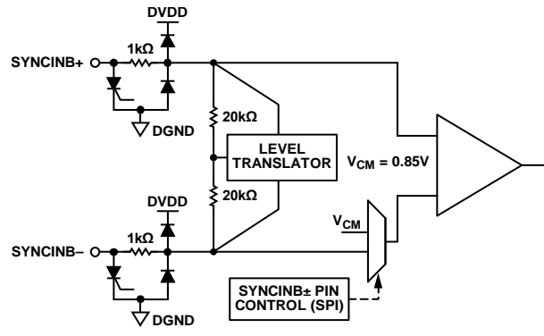
Figure 108. SYNCINB± Inputs
