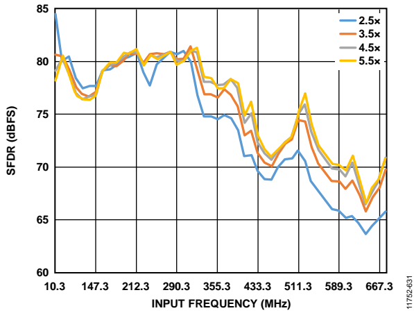
Figure 118. Buffer Current Sweeps, AD9680-1250 (SFDR vs. I_{BUFF} ); f_{IN} < 500\text{ MHz} ; Front-End Network Shown in Figure 115
