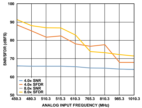
Figure 91. SNR/SFDR vs. f_{IN} ; 500 MHz < f_{IN} < 1 GHz; Buffer Control 1 (0x018) = 4.0x and 8.0x
