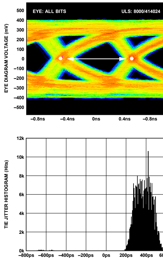
Figure 52. Data Eye for LVDS Outputs in ANSI-644 Mode with Trace Lengths of Greater Than 24 Inches on Standard FR-4 Material, External 100 \Omega Far End Termination Only
