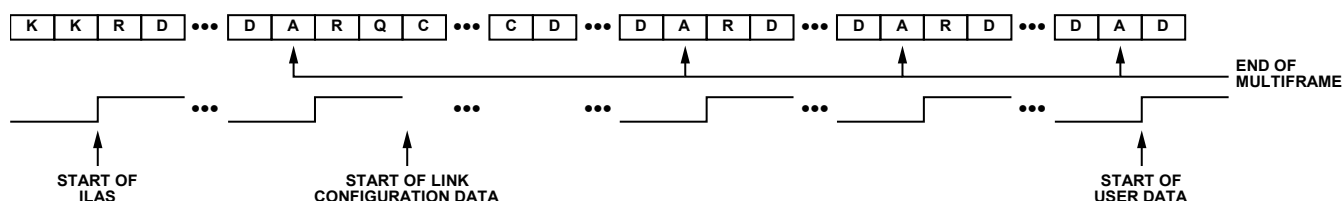
Figure 134. Initial Lane Alignment Sequence
