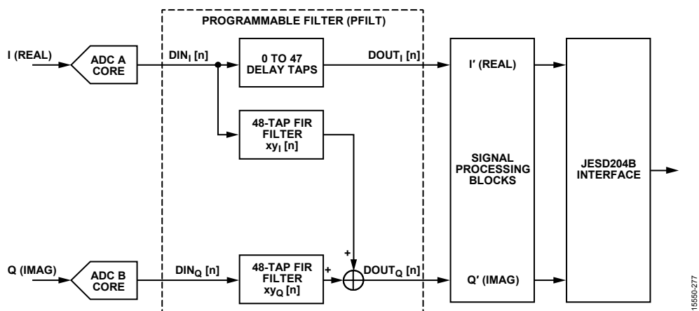
Figure 107. 48-Tap Half Complex Filter Configuration
