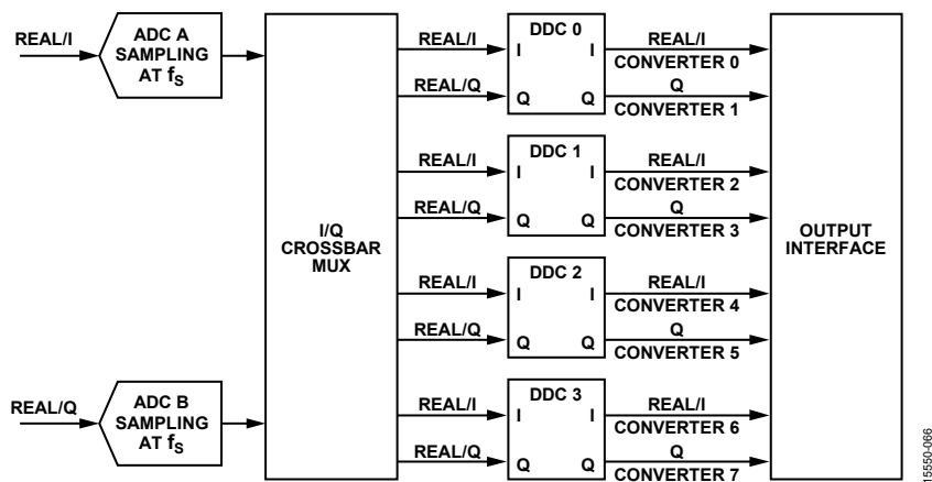
Figure 102. DDCs and Virtual Converter Mapping
