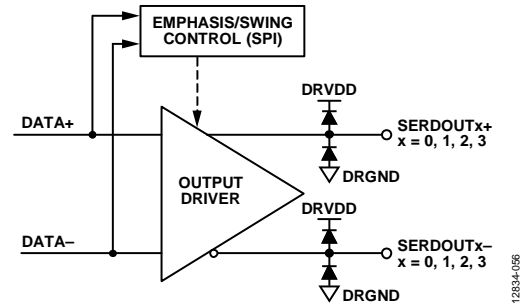
Figure 56. Digital Outputs
