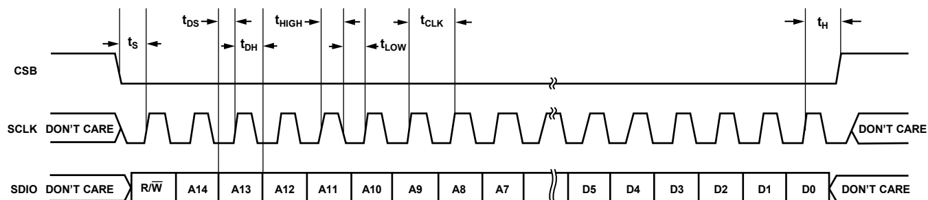
Figure 3. SPI Timing Diagram
