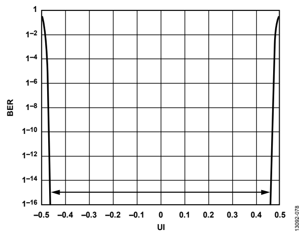
Figure 77. Digital Outputs Bathtub Curve, External 100\ \Omega Terminations at 6 Gbps
