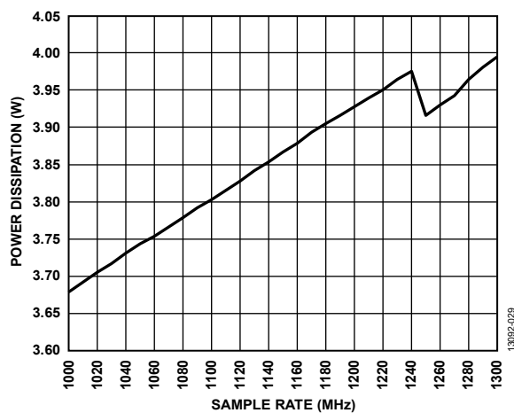
Figure 29. Power Dissipation vs. Sample Rate ( f_s )
