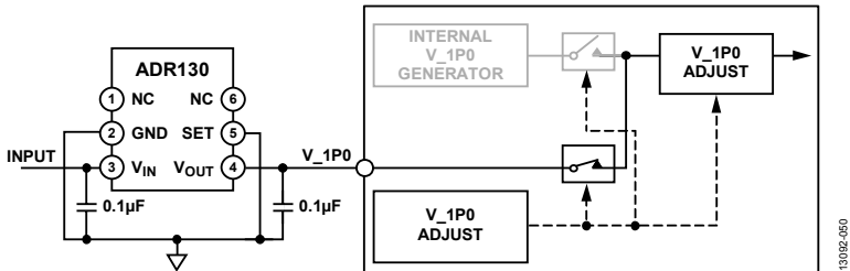
Figure 49. External Reference Using the ADR130
