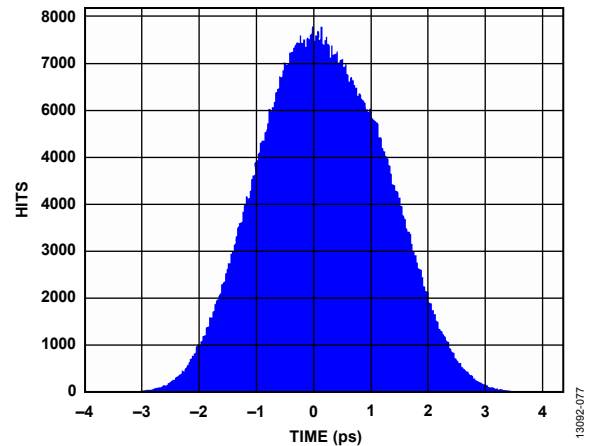
Figure 76. Digital Outputs Histogram, External 100\ \Omega Terminations at 6 Gbps
