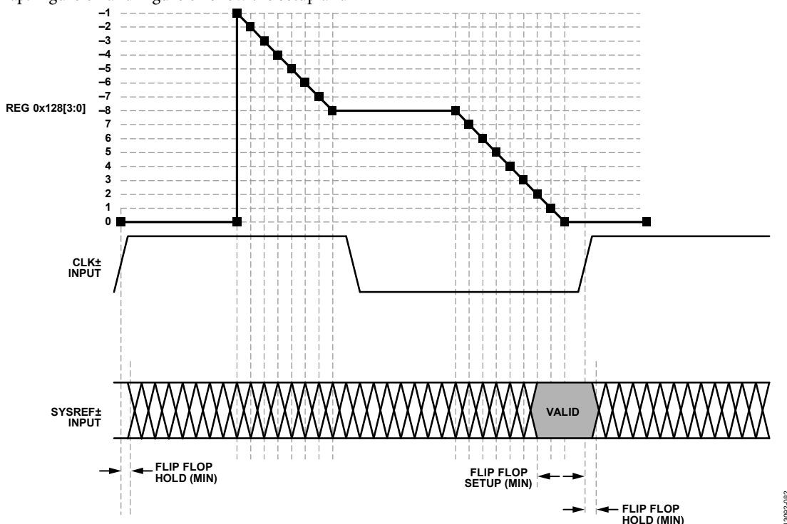
Figure 81. SYSREF± Setup Detector
