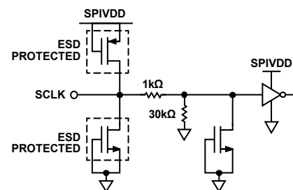
Figure 35. SCLK Input
