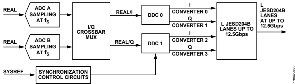
Figure 79. Two-ADC Plus Two-DDC Mode
