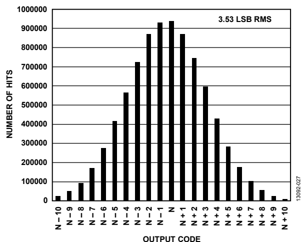
Figure 27. Input Referred Noise Histogram
