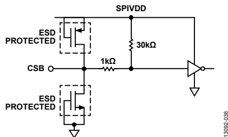
Figure 36. CSB Input
