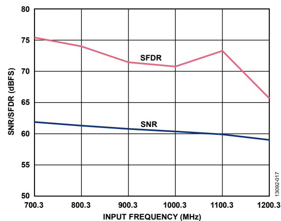
Figure 17. SNR/SFDR vs. Input Frequency ( f_{IN} ), 700\text{ MHz} < f_{IN} < 1200 MHz, Buffer Current = 4.5\times (See Figure 41 and Table 9)
