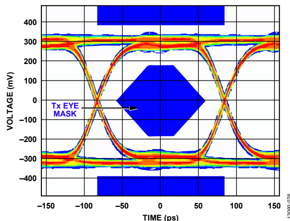
Figure 75. Digital Outputs Data Eye, External 100\ \Omega Terminations at 6 Gbps
