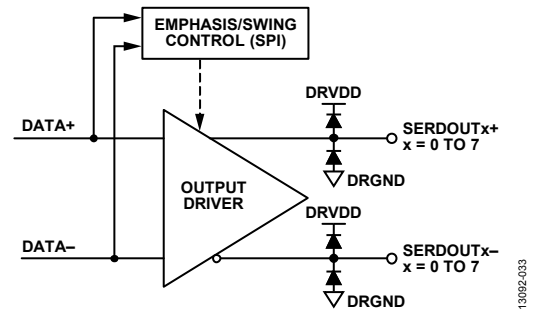
Figure 33. Digital Outputs
