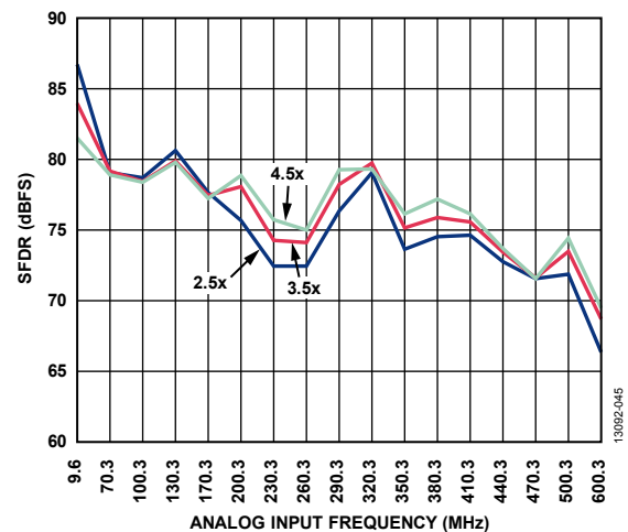
Figure 44. Buffer Current Sweeps, SFDR vs. Analog Input Frequency vs. I_{BUFF} ; f_{IN} < 600 \text{ MHz}
