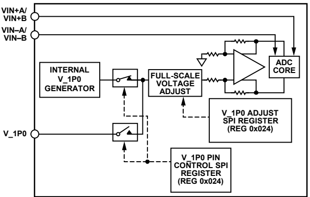
Figure 47. Internal Reference Configuration and Controls
