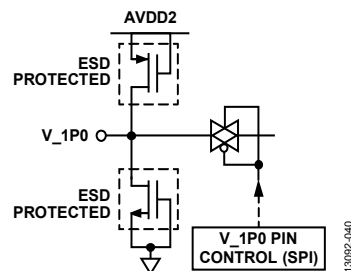
Figure 40. V_1P0 Input
