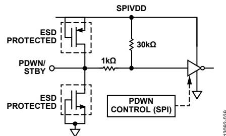
Figure 39. PDWN/STBY Input
