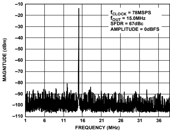
Figure 51. AD9704 Single-Tone SFDR
