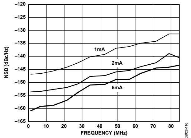
Figure 16. NSD vs. f_{OUT} and I_{OUT} @ 175 MSPS
