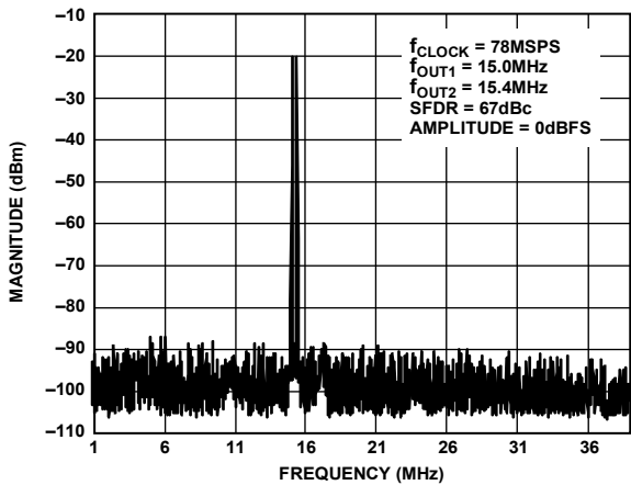
Figure 52. AD9704 Dual-Tone SFDR
