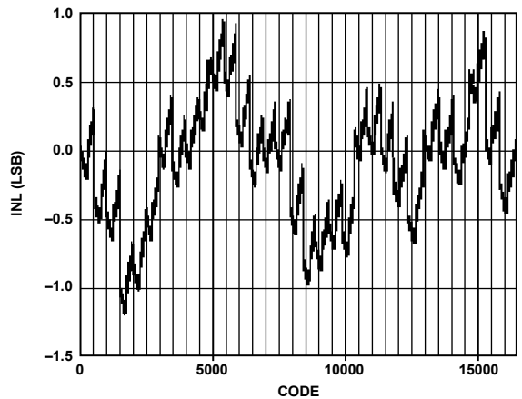
Figure 38. Typical Uncalibrated INL
