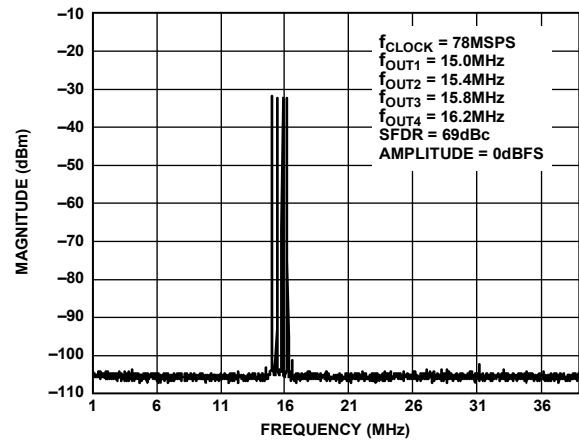
Figure 43. Four-Tone SFDR
