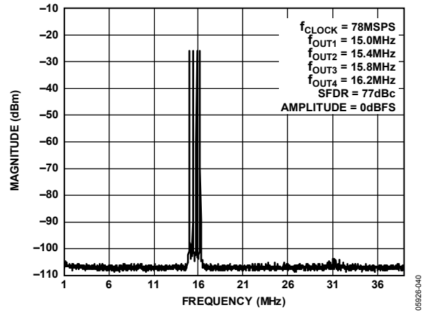
Figure 26. Four-Tone SFDR
