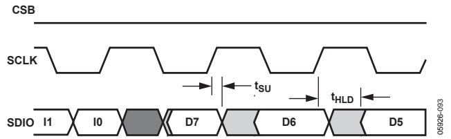
Figure 77. Timing Diagram for SPI Register Read
