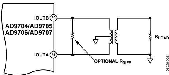
Figure 88. Differential Output Using a Transformer
