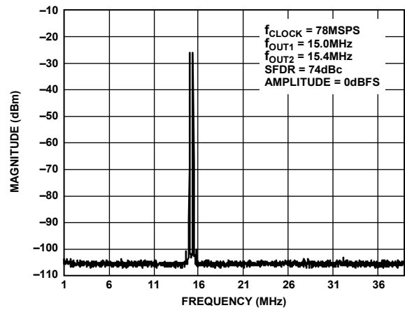
Figure 42. Dual-Tone SFDR
