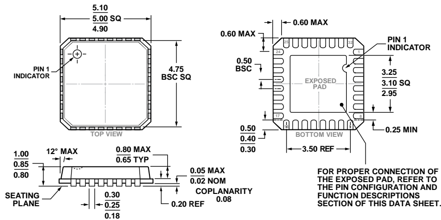
Figure 91. 32-Lead Lead Frame Chip Scale Package [LFCSP] 5 mm × 5 mm and 0.85 mm Package Height (CP-32-2)
