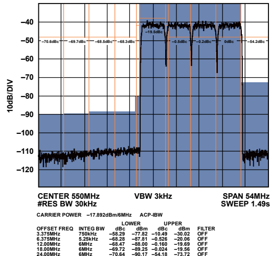
Figure 52. Mid Band Narrow-Band ACLR (Worse Side)
