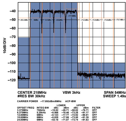
Figure 51. Low Band Narrow-Band ACLR (Worse Side)
