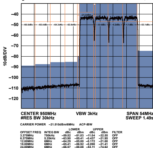
Figure 53. High Band Narrow-Band ACLR (Worse Side)
