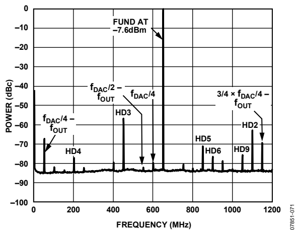
Figure 70. Spectral Plot
