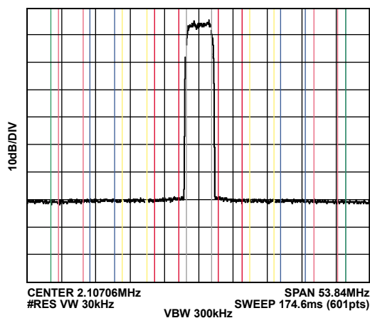
Figure 27. Typical Single-Carrier WCDMA ACLR Performance at 2.1 GHz, f_{DAC} = 2457.6 MSPS (Second Nyquist Zone)
