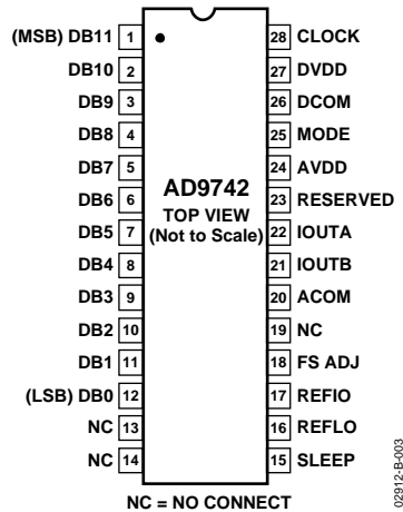
Figure 3. 28-Lead SOIC and 28-Lead TSSOP Pin Configuration
