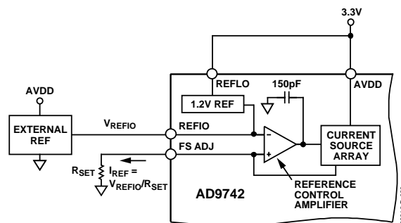
Figure 24. External Reference Configuration
