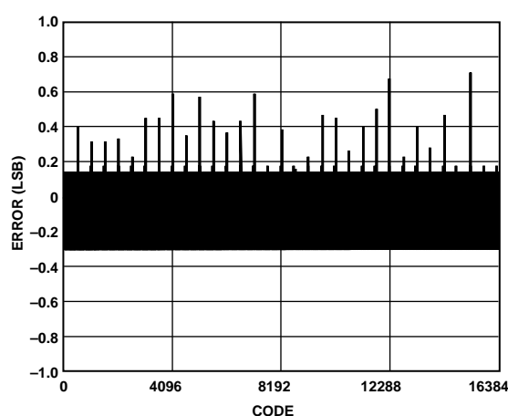
Figure 16. Typical DNL
