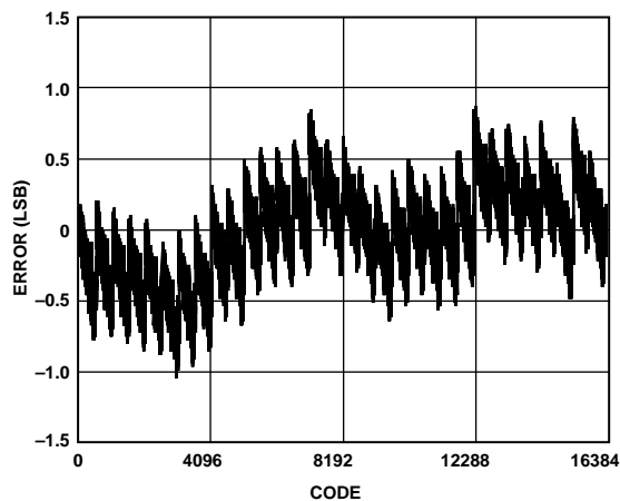
Figure 15. Typical INL
