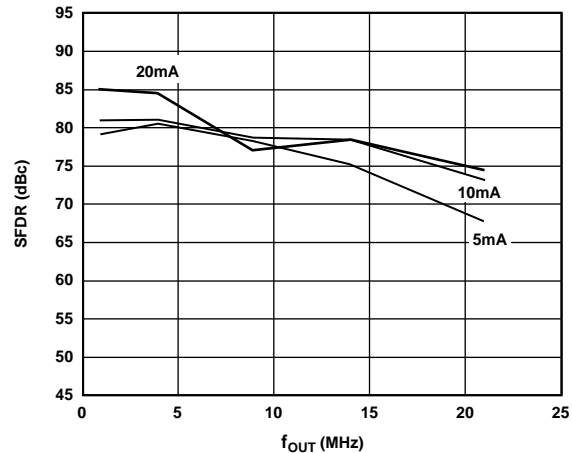
Figure 10. SFDR vs. f_{OUT} and I_{OUT} at 65 MSPS and 0 dBFS
