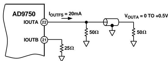
Figure 31. 0 V to +0.5 V Unbuffered Voltage Output
