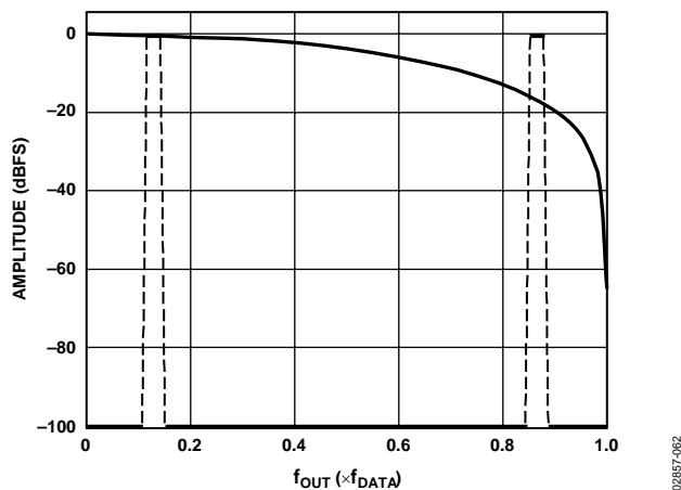
Figure 62. No Interpolation, Modulation = f_{\text{DAC}}/8
