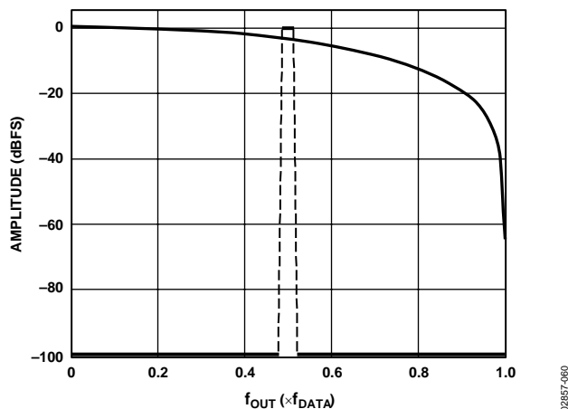
Figure 60. No Interpolation, Modulation = f_{\text{DAC}}/2
