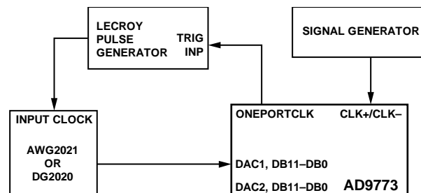
JUMPER CONFIGURATION FOR ONE-PORT MODE, PLL ON
