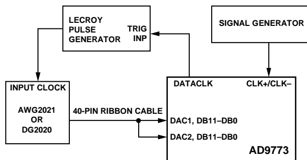
JUMPER CONFIGURATION FOR TWO-PORT MODE, PLL ON
