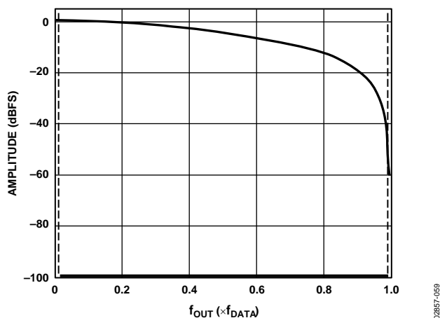
Figure 59. No Interpolation, Modulation Disabled
