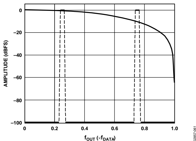
Figure 61. No Interpolation, Modulation = f_{\text{DAC}}/4
