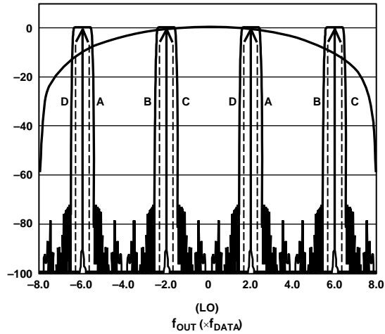
Figure 85. 8× Interpolation, Complex f_{DAC}/4 Modulation
