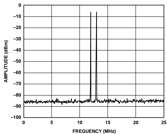
Figure 29. Two-Tone IMD Performance, f_{OUT} = 10 MHz, f_{DATA} = 50 MSPS, Interpolation = 8×
