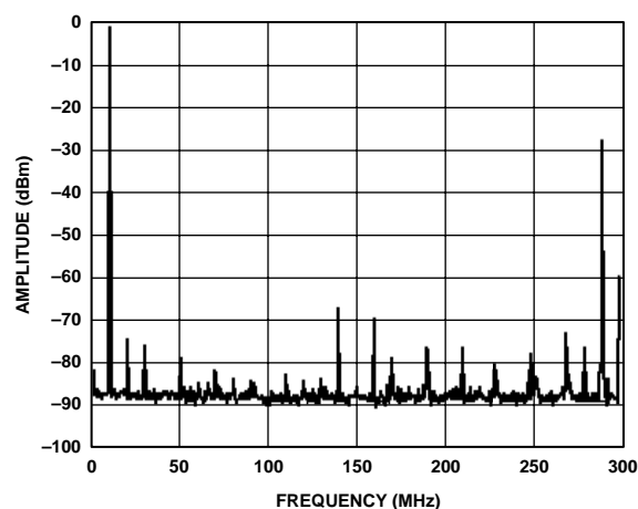
Figure 26. Single-Tone Spurious Performance, f_{OUT} = 10 MHz, f_{DATA} = 150 MSPS, Interpolation = 2×
