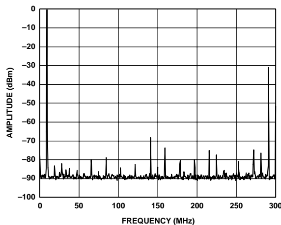
Figure 28. Single-Tone Spurious Performance, f_{OUT} = 10 MHz, f_{DATA} = 80 MSPS, Interpolation = 4×
