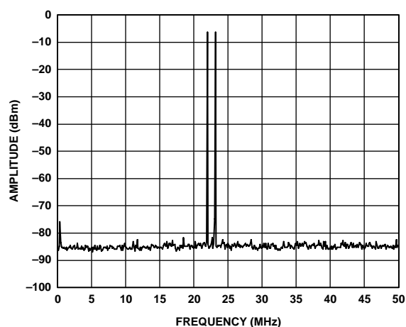
Figure 27. Two-Tone IMD Performance, f_{DATA} = 150 MSPS, Interpolation = 4×
