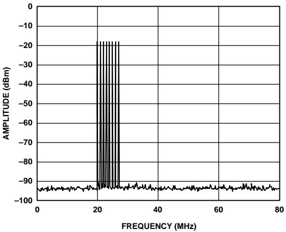
Figure 31. Eight-Tone IMD Performance, f_{DATA} = 160\text{ MSPS} , Interpolation = 8\times
