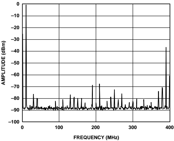
Figure 30. Single-Tone Spurious Performance, f_{OUT} = 10\text{ MHz} , f_{DATA} = 50\text{ MSPS} , Interpolation = 8\times
