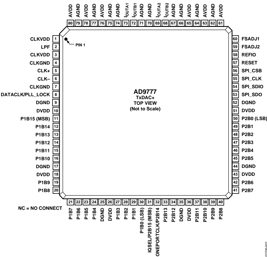
Figure 5. Pin Configuration
