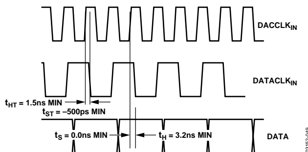
Figure 49. Slave Mode Timing, 2× Interpolation, DCLKPOL = 0
