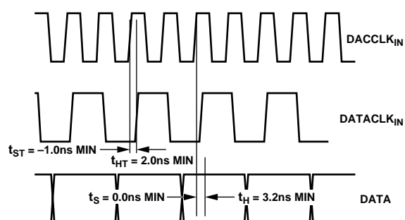
Figure 50. Slave Mode Timing, 2× Interpolation, DCLKPOL = 1
