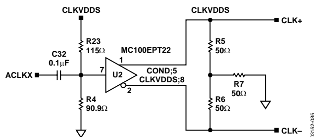
Figure 85. PECL Driver on AD9786 Rev. F Evaluation Board
