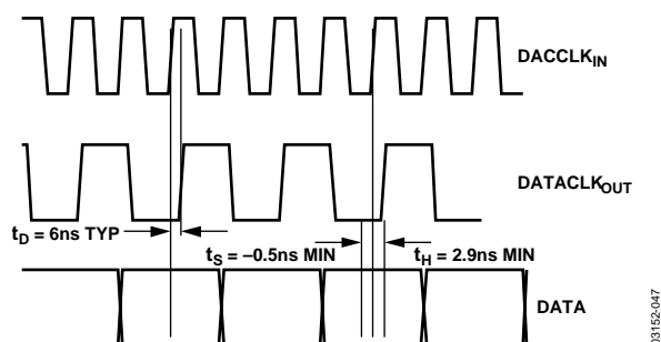
Figure 47. Data Timing, 2× Interpolation, DCLKPOL = 0
