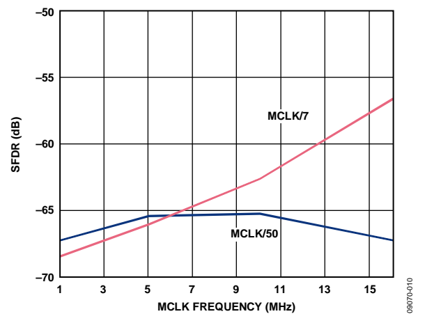
Figure 9. Wideband SFDR vs. MCLK Frequency
